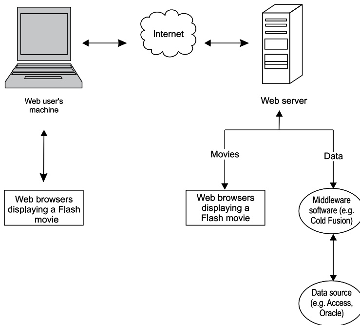
Figure 2-1: A dynamic data workflow.
